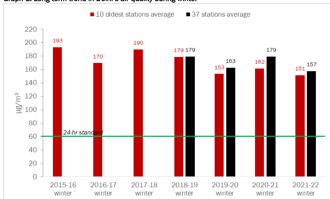
Graph 1: Long term trend in Delhi's air quality during winter
