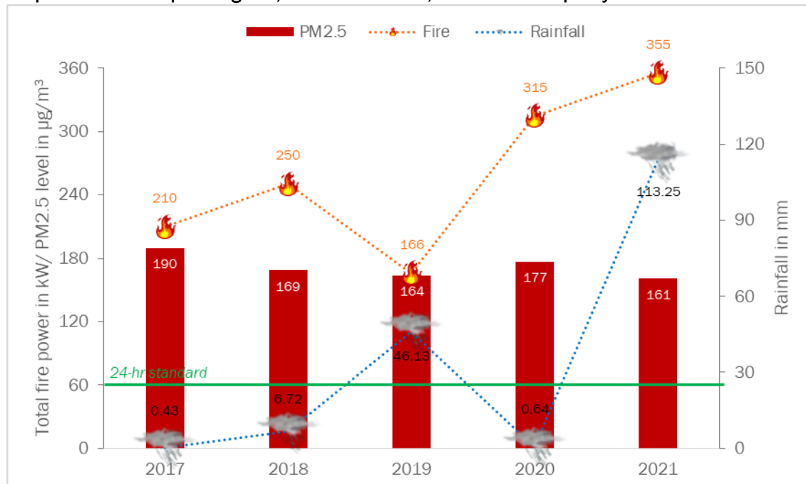
Graph 6: Relationship among rain, farm stubble fires, and Delhi's air quality in October-November
