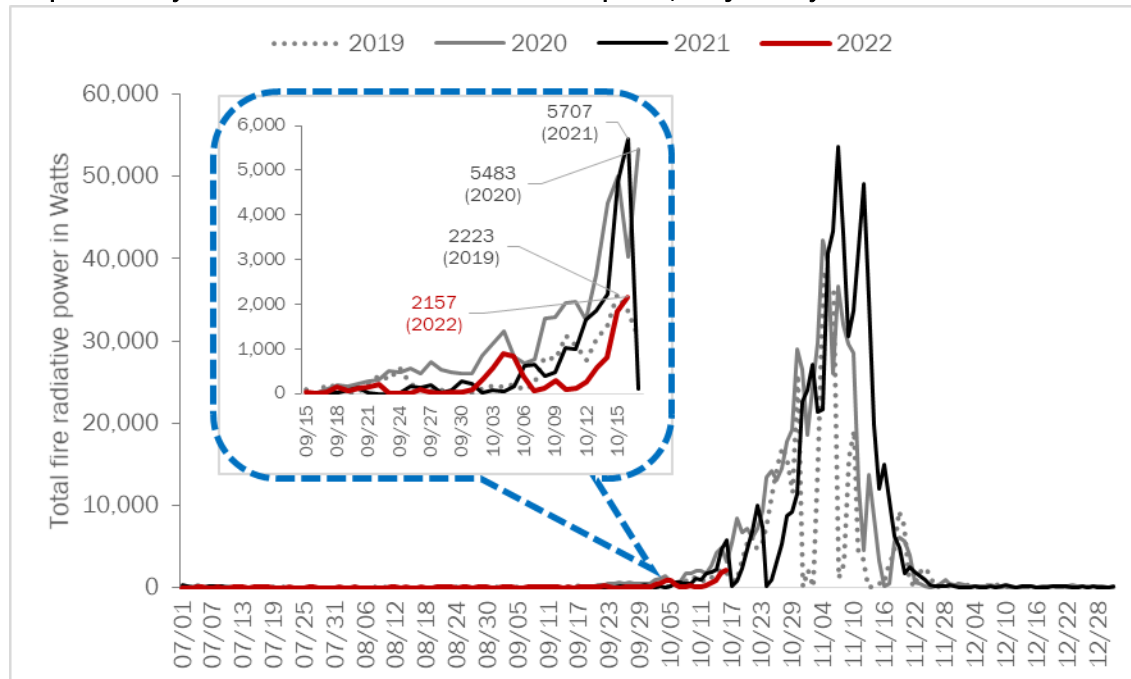
Graph 15: Daily trend of farm stubble fire's radiative power, Punjab-Haryana-Delhi
