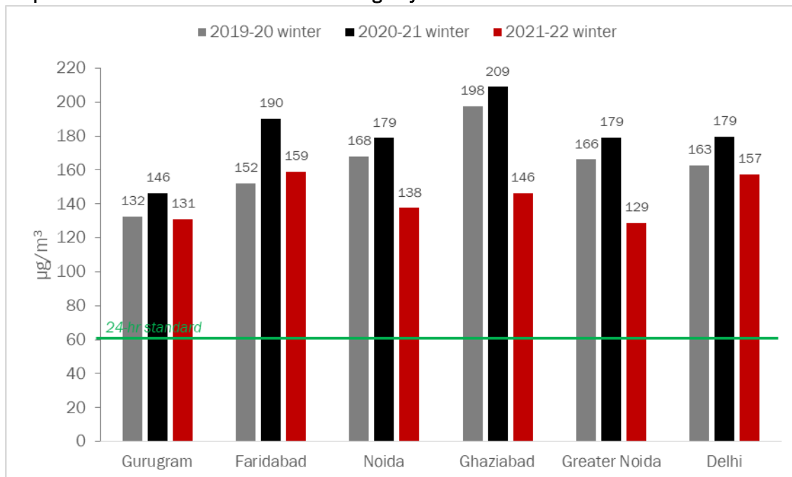
Graph 3: Last three winter's PM 2.5 level among major cities of core NCR
