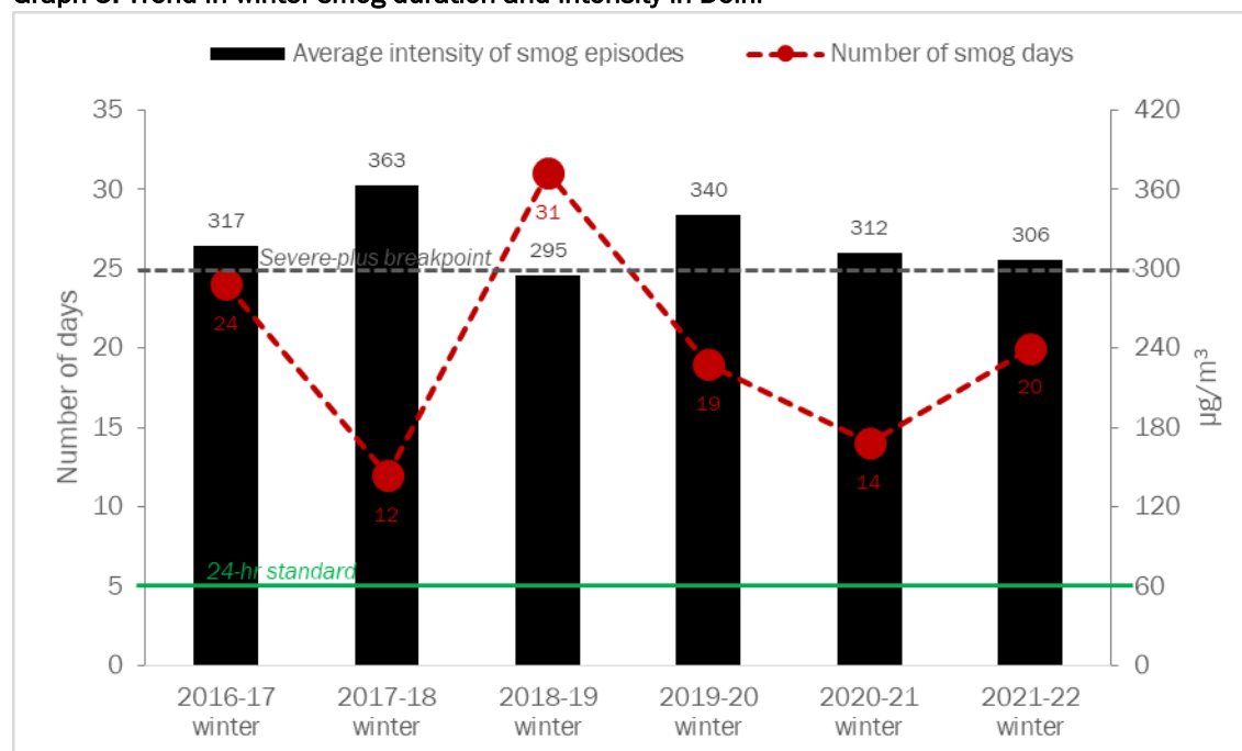
Graph 5: Trend in winter smog duration and intensity in Delhi
