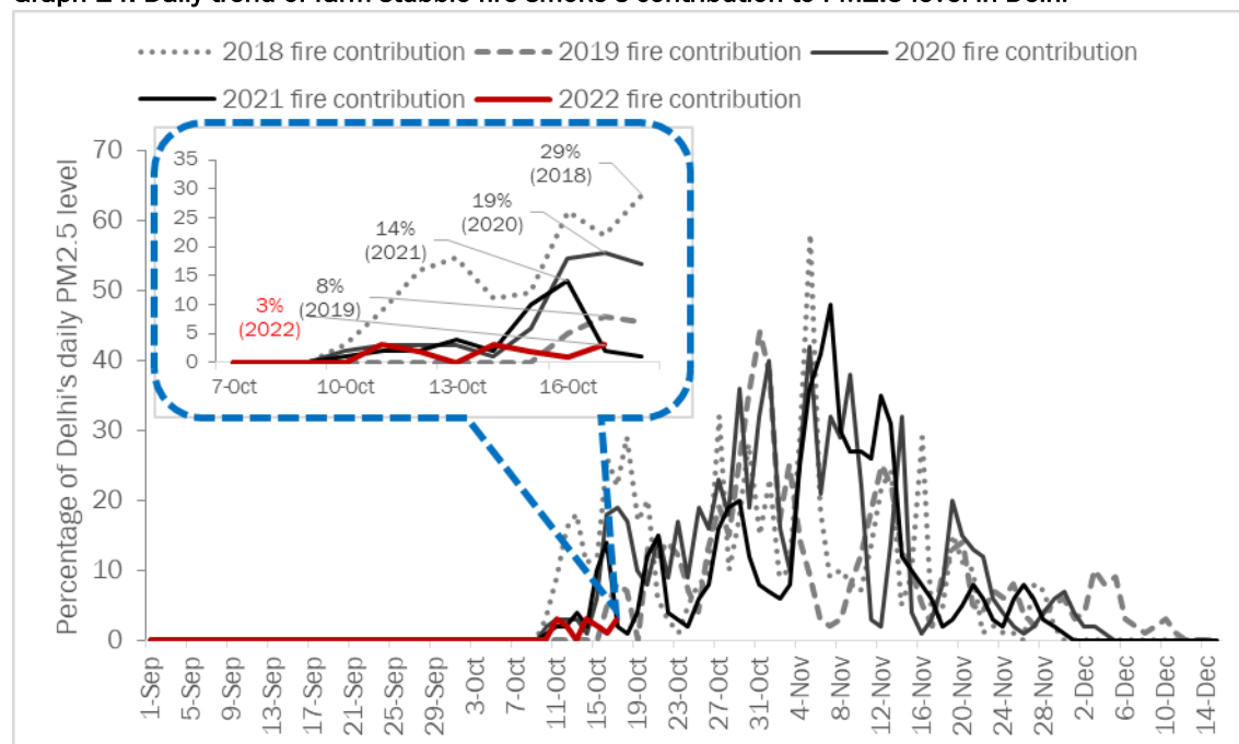
Graph 14: Daily trend of farm stubble fire smoke's contribution to PM2.5 level in Delhi
