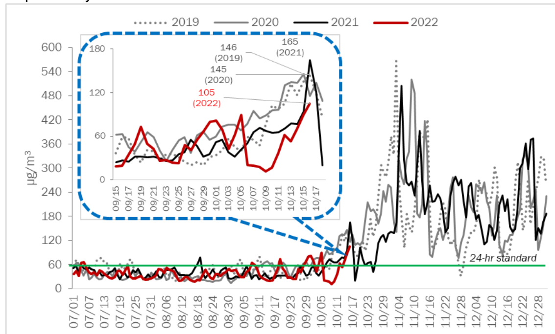
Graph 13: Daily trend of PM2.5 level in Delhi
