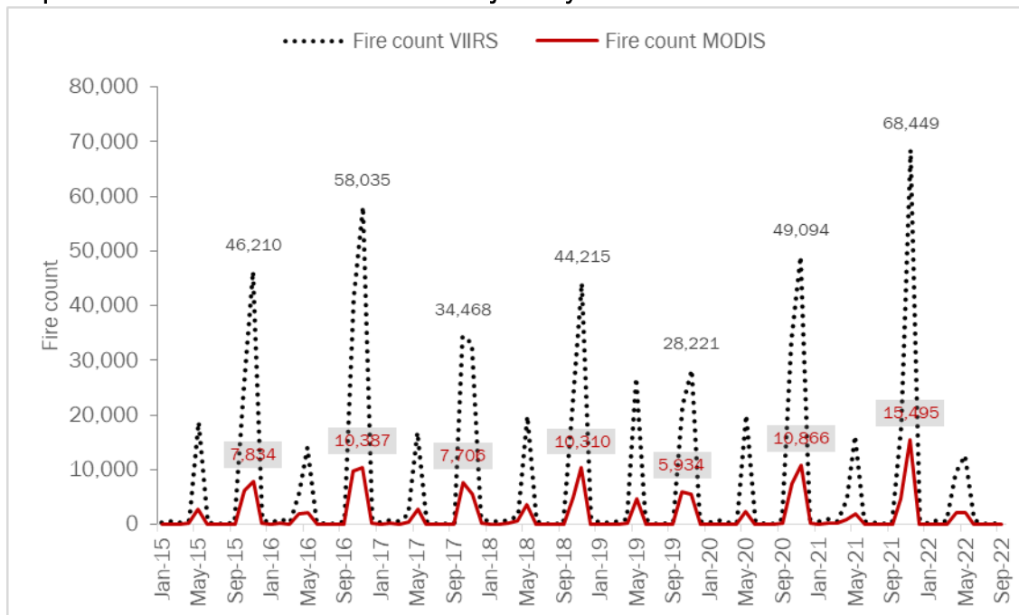
Graph 7: Trend in farm stubble fire count in Punjab-Haryana-Delhi 2015-22
