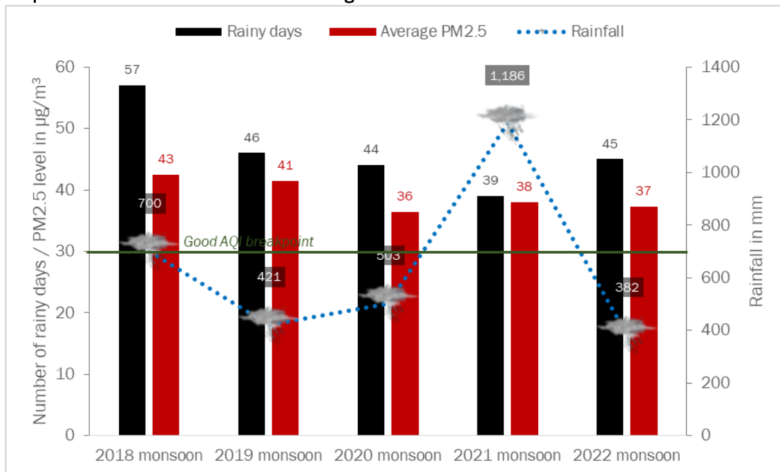
Graph 10: Trend in PM2.5 and rainfall during monsoon season in Delhi
