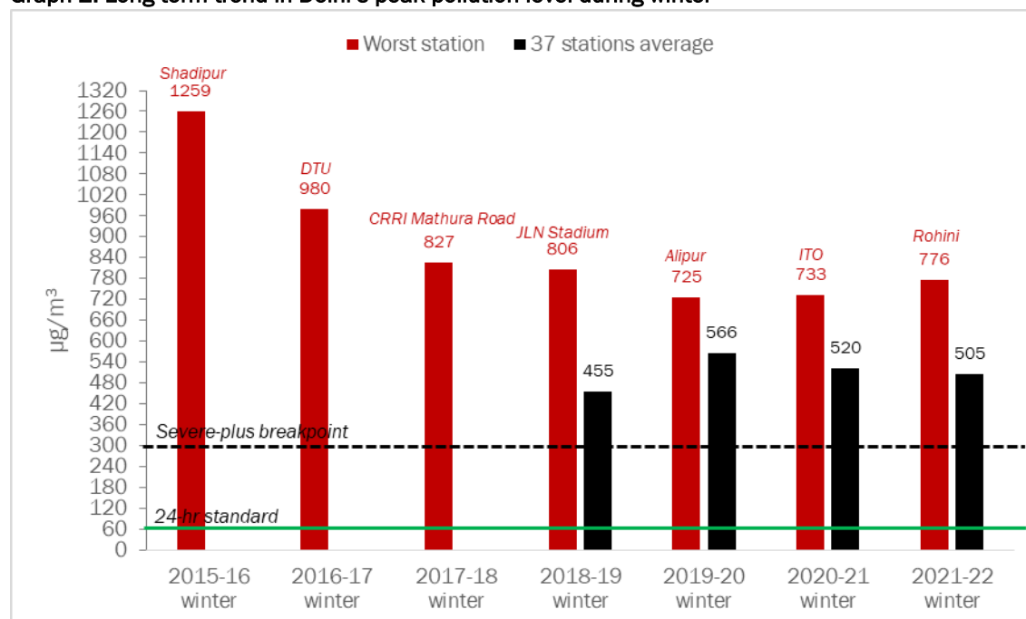
Graph 2: Long term trend in Delhi's peak pollution level during winter
