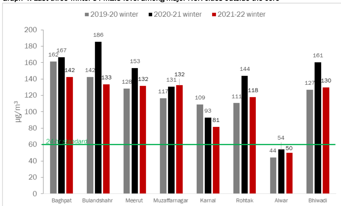
Graph 4: Last three winter's PM 2.5 level among major NCR cities outside the core
