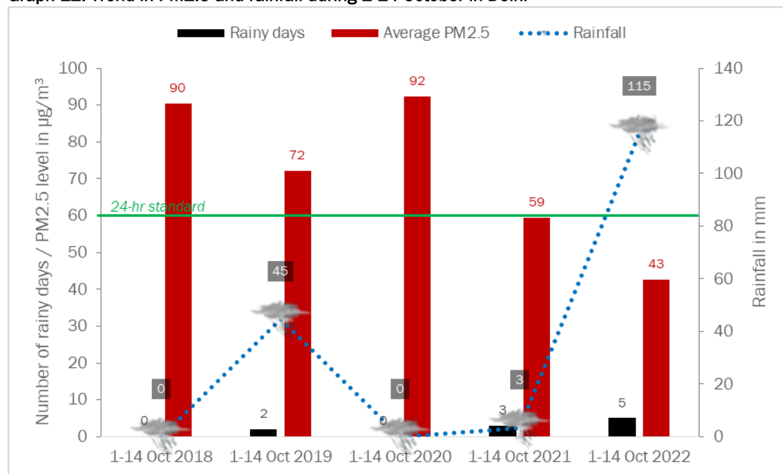
Graph 12: Trend in PM 2.5 and rainfall during 1-14 October in Delhi
