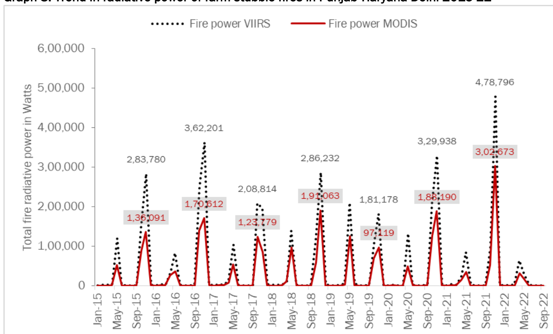
Graph 8: Trend in radiative power of farm stubble fires in Punjab-Haryana-Delhi 2015-22
