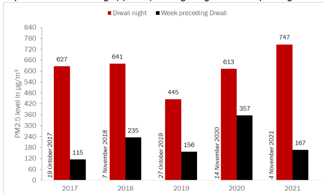
Graph 9: PM 2.5 levels Diwali-night (8pm-8am) vs average of nights in the week preceding Diwali
