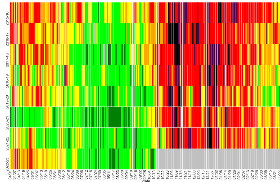
Graph 11: Air quality heatmap of Delhi
