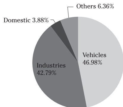
Graph 18: Sources of NOx (2007)
