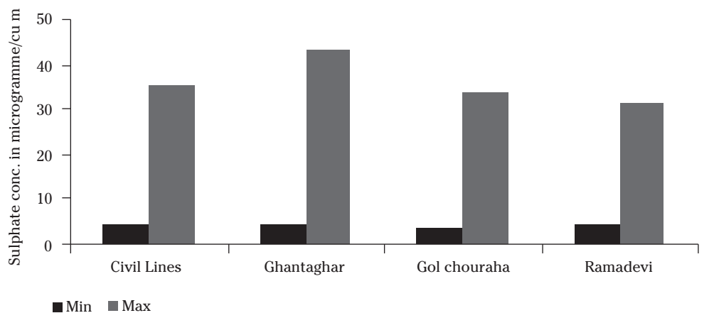
Graph 12: Sulphate concentration in various locations of Kanpur
