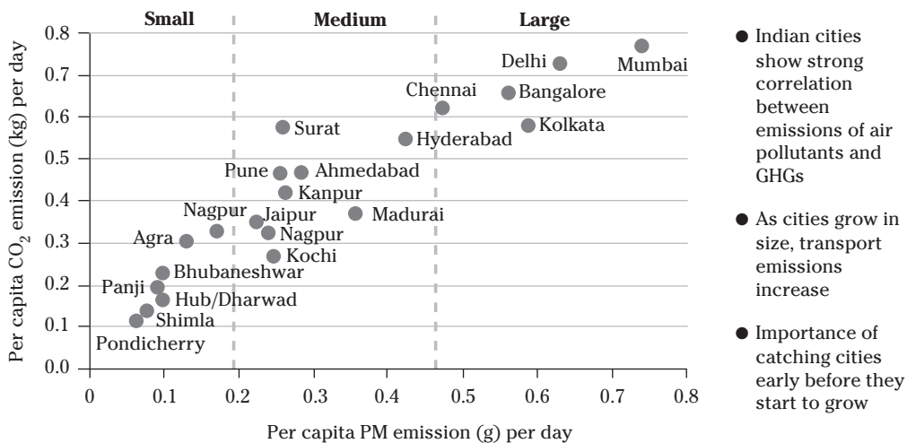
Graph 3: Per capita PM and CO 2 in cities
