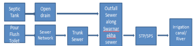
Figure 1: Schematic sketch of wastewater collection, conveyance and disposal system (UD&ED, 2010)
