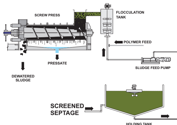
Figure 4: Typical mechanical septage dewatering system
